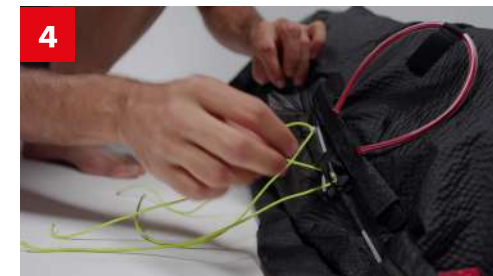
4 Pass both wires through the holes prepared
